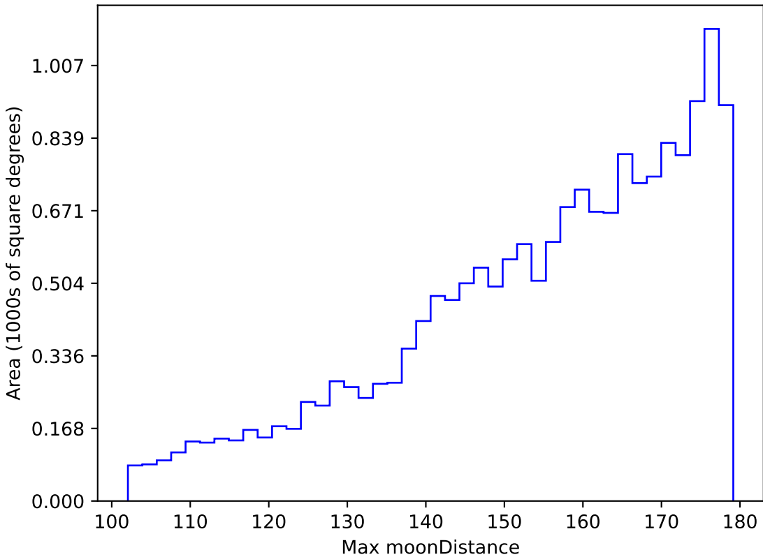
too_ignore_5_4v3.4_10yrs WFD u band: Max moonDistance
