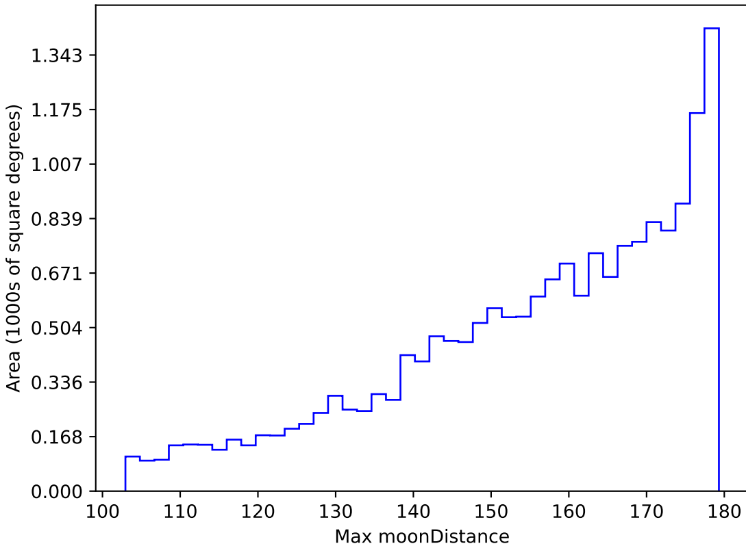
too_ignore_5_4v3.4_10yrs WFD i band: Max moonDistance
