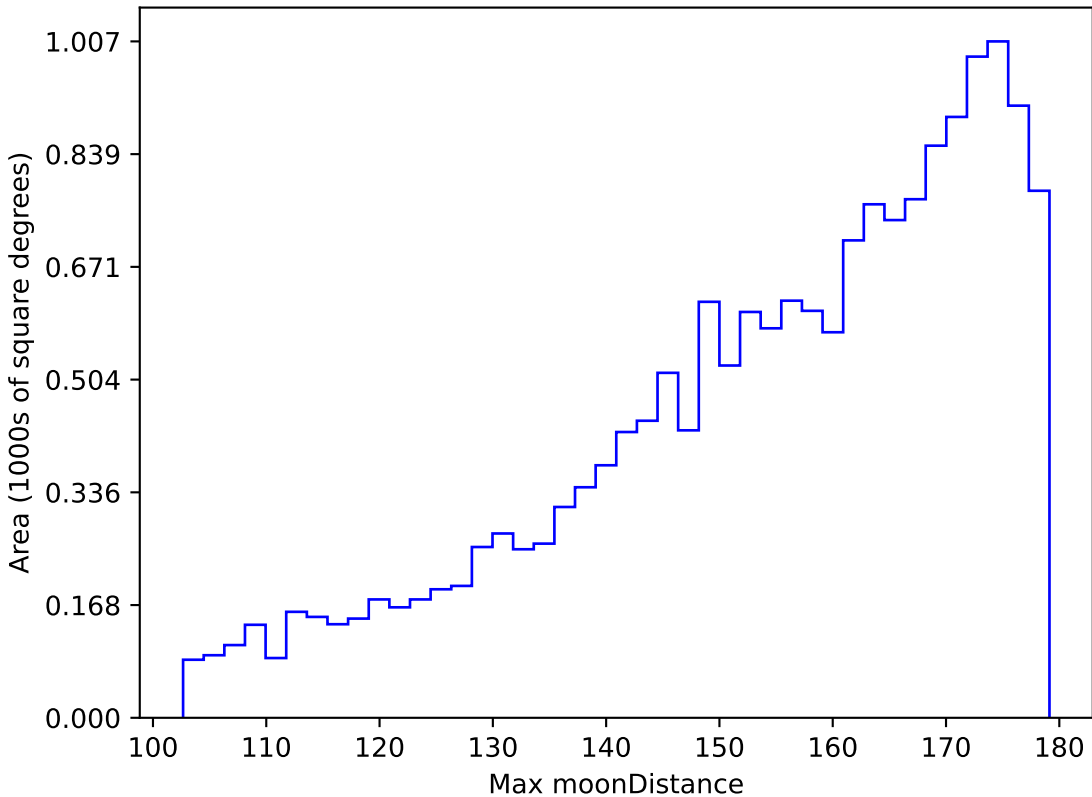
too_ignore_5_4v3.4_10yrs WFD g band: Max moonDistance
