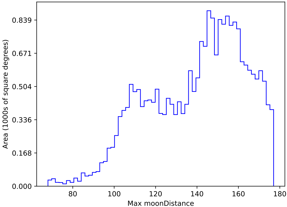
too_ignore_5_4v3.4_10yrs All sky y band: Max moonDistance
