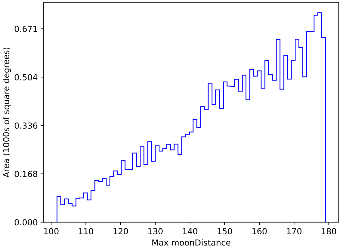
too_ignore_5_4v3.4_10yrs All sky u band: Max moonDistance
