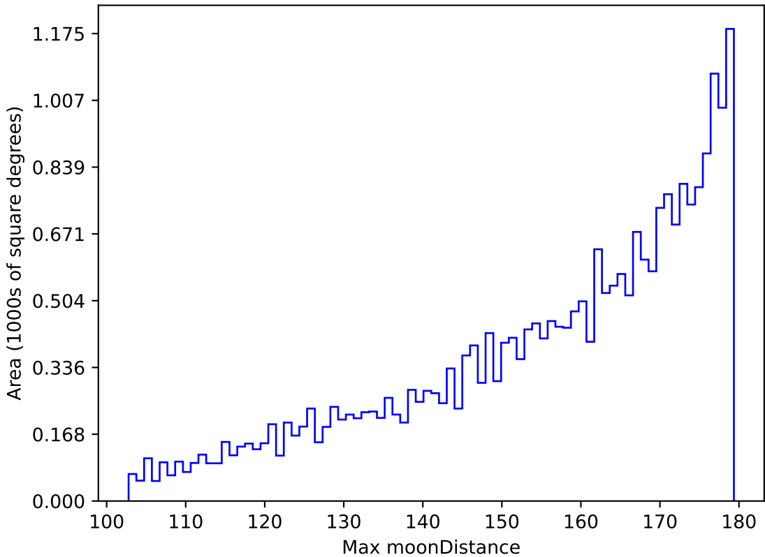
too_ignore_5_4v3.4_10yrs All sky r band: Max moonDistance
