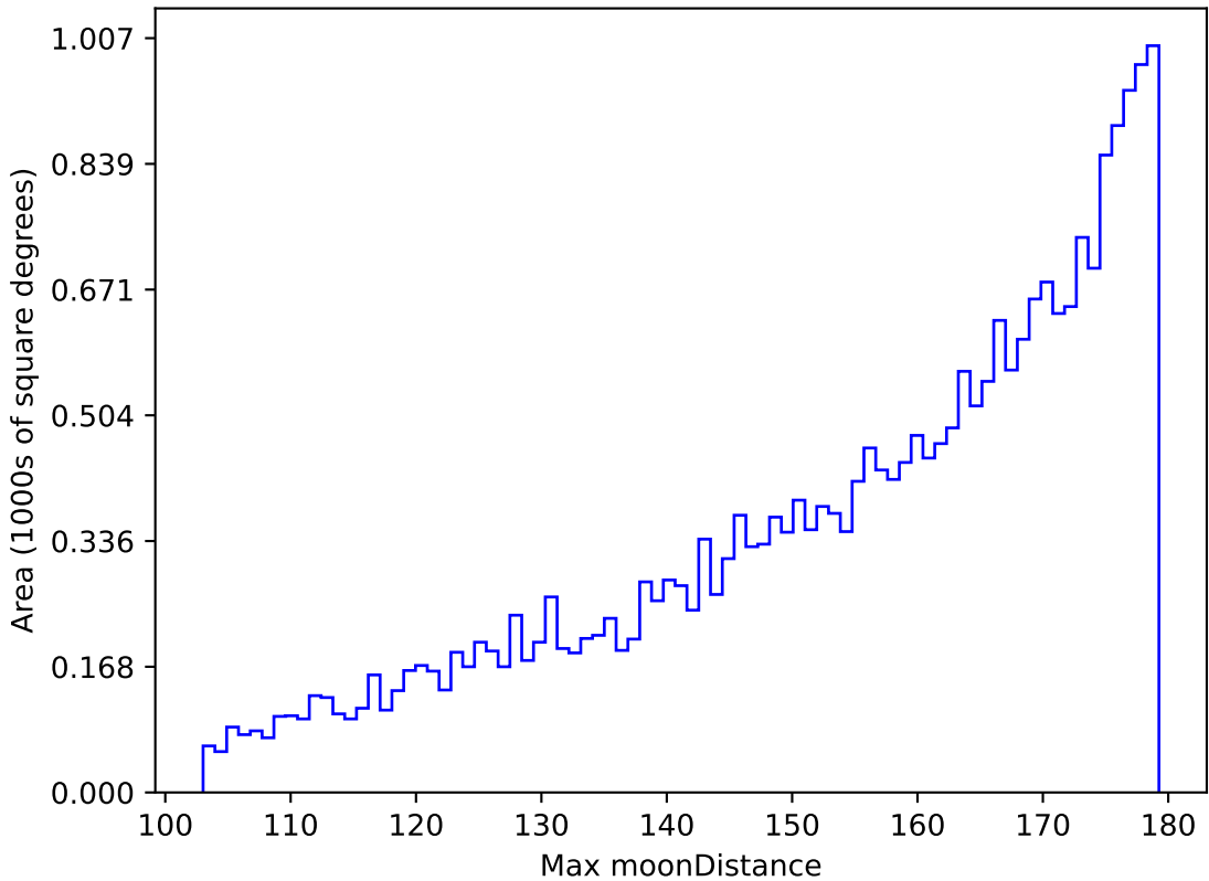
too_ignore_5_4v3.4_10yrs All sky i band: Max moonDistance
