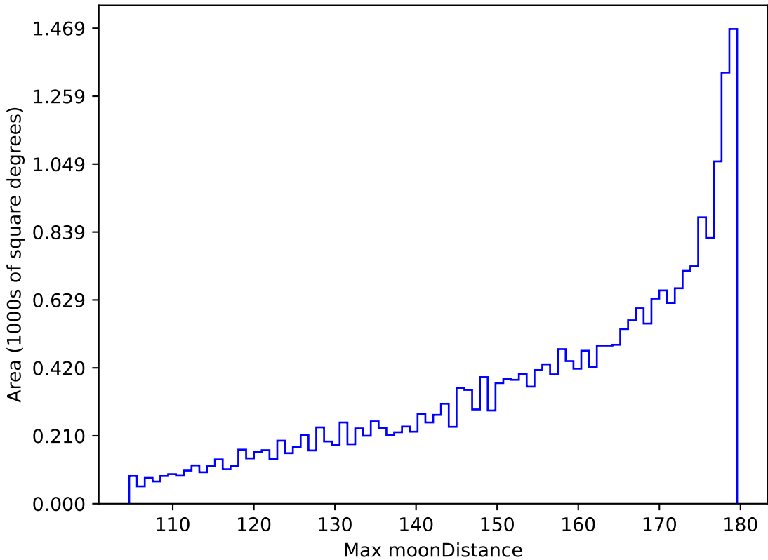
too_ignore_5_4v3.4_10yrs All sky all bands: Max moonDistance
