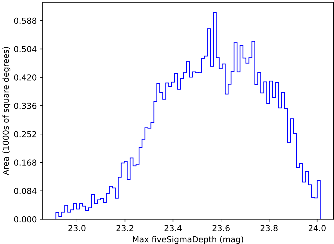
too_ignore_5_4v3.4_10yrs Yr 1 u band: Max fiveSigmaDepth
