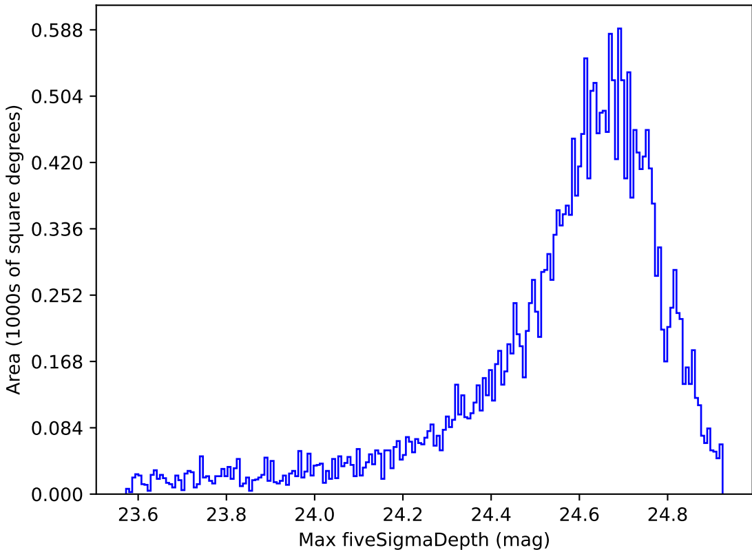
too_ignore_5_4v3.4_10yrs Yr 1 r band: Max fiveSigmaDepth
