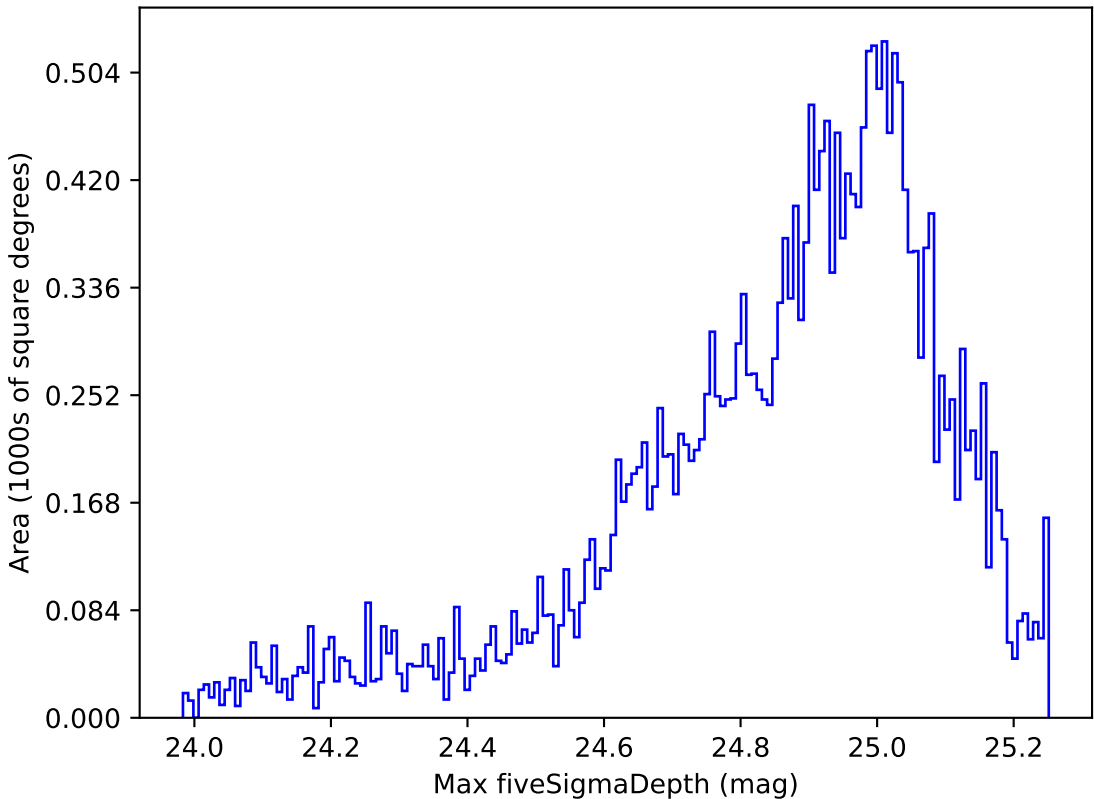
too_ignore_5_4v3.4_10yrs Yr 1 g band: Max fiveSigmaDepth
