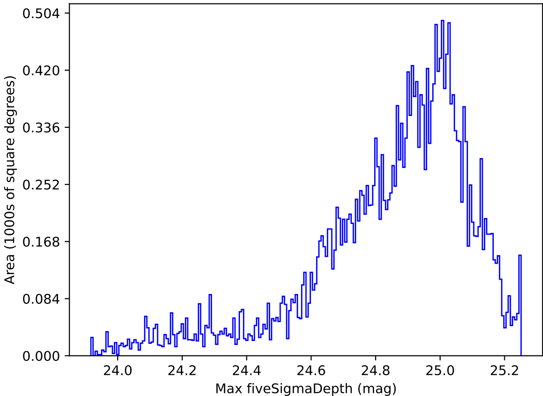
too_ignore_5_4v3.4_10yrs Yr 1 all bands: Max fiveSigmaDepth
