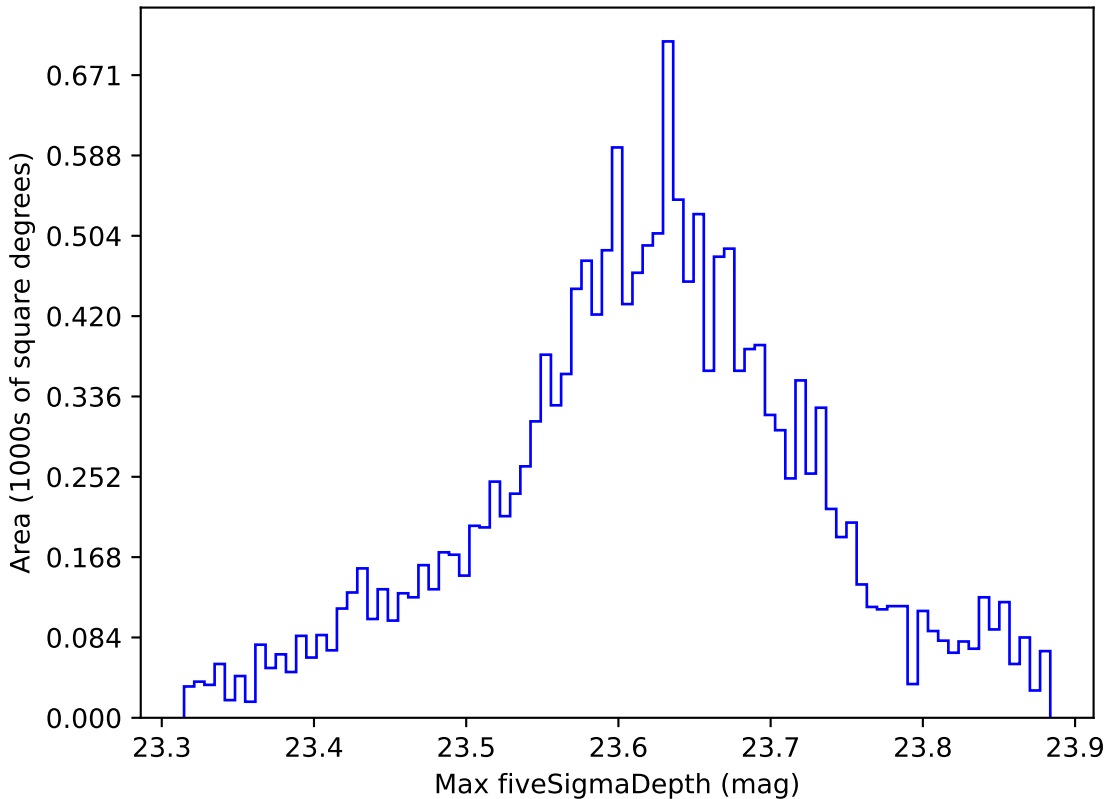
too_ignore_5_4v3.4_10yrs WFD z band: Max fiveSigmaDepth
