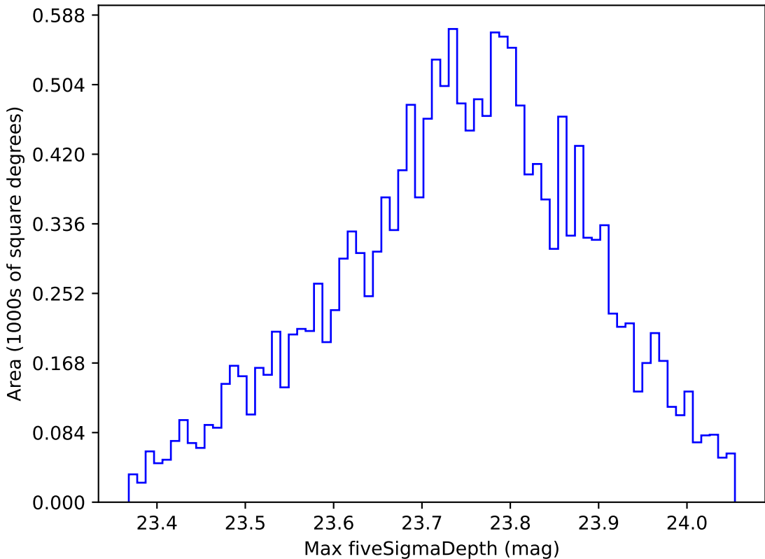
too_ignore_5_4v3.4_10yrs WFD u band: Max fiveSigmaDepth
