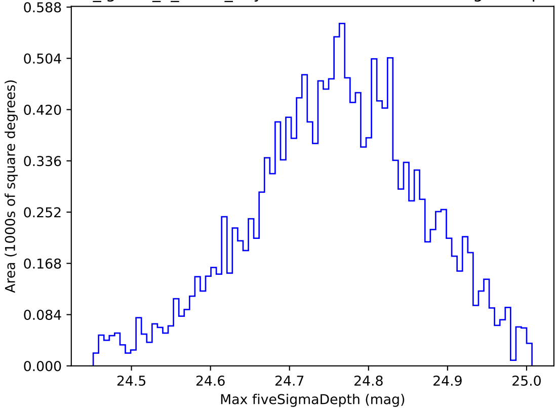
too_ignore_5_4v3.4_10yrs WFD r band: Max fiveSigmaDepth
