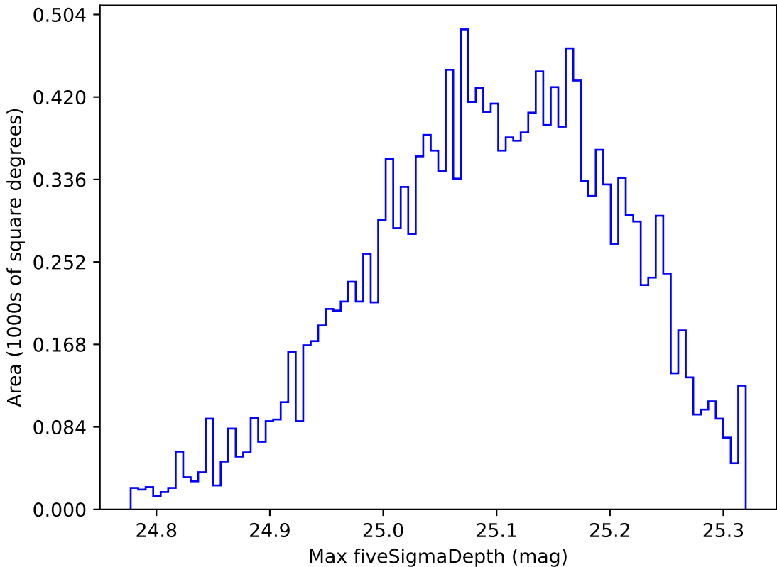
too_ignore_5_4v3.4_10yrs WFD g band: Max fiveSigmaDepth
