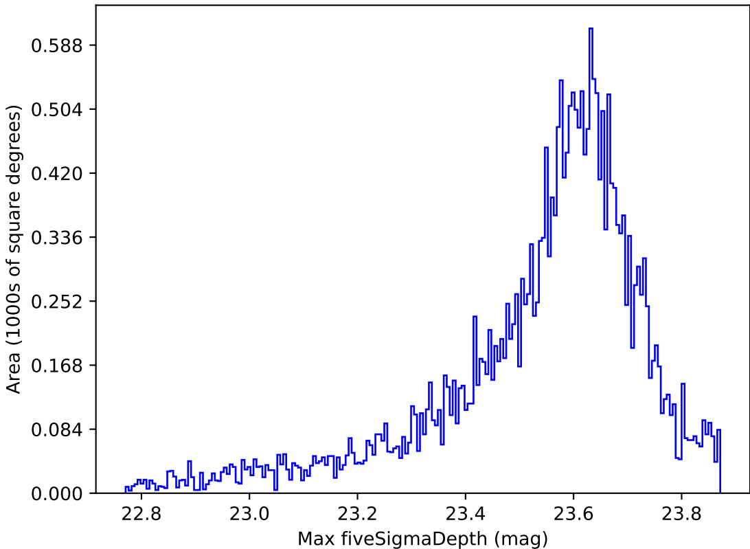
too_ignore_5_4v3.4_10yrs All sky z band: Max fiveSigmaDepth
