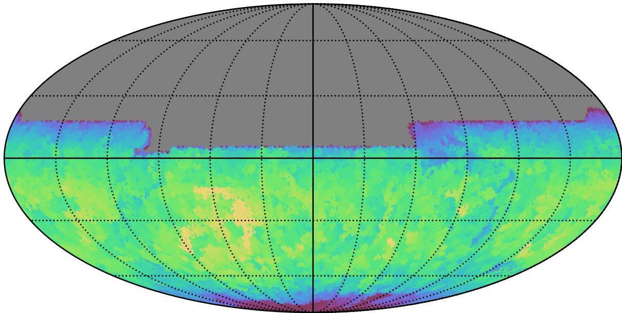
too_ignore_5_4v3.4_10yrs All sky y band: Max fiveSigmaDepth
