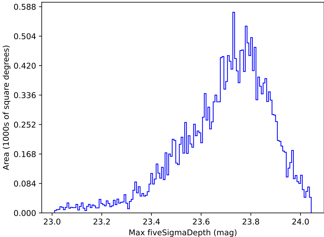
too_ignore_5_4v3.4_10yrs All sky u band: Max fiveSigmaDepth
