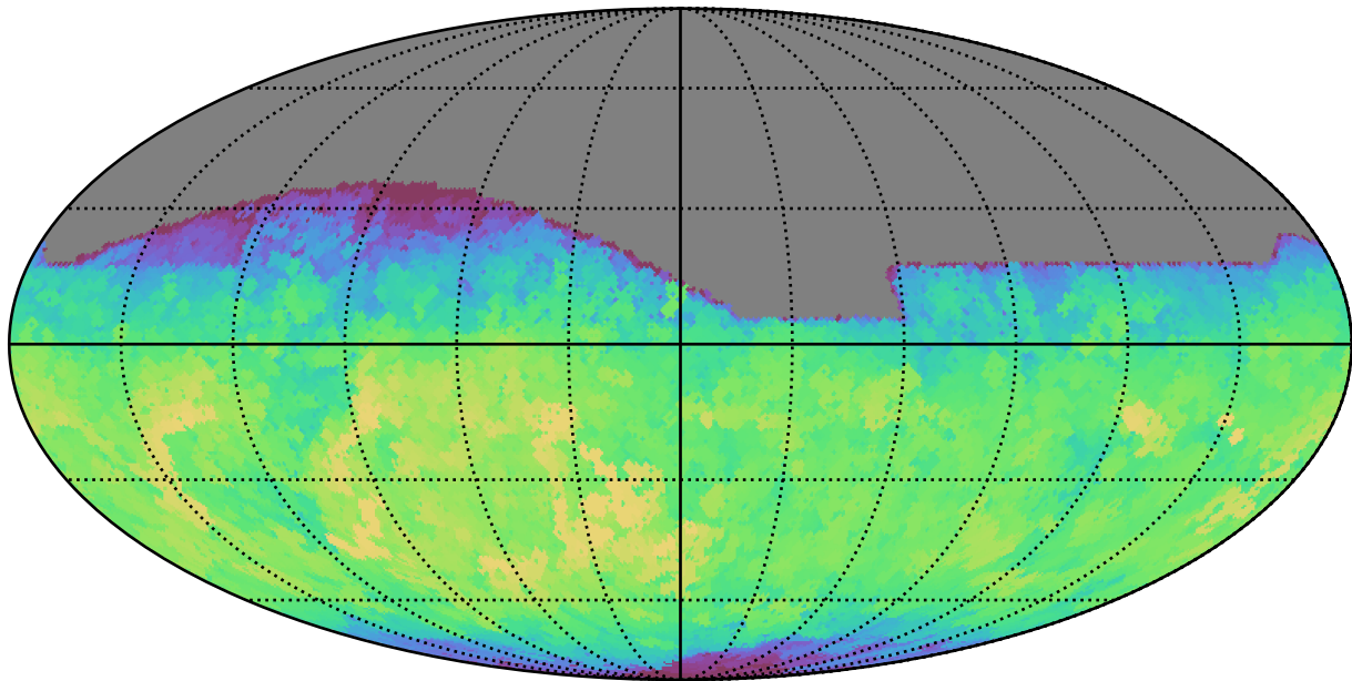
too_ignore_5_4v3.4_10yrs All sky i band: Max fiveSigmaDepth
