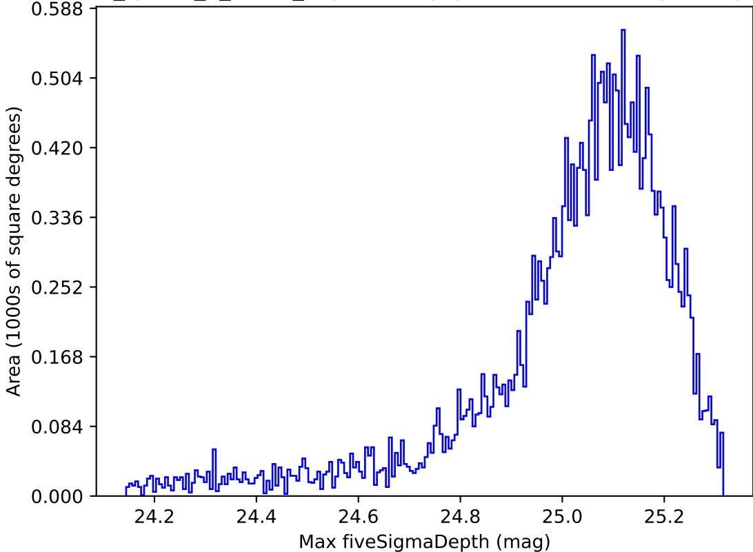
too_ignore_5_4v3.4_10yrs All sky g band: Max fiveSigmaDepth
