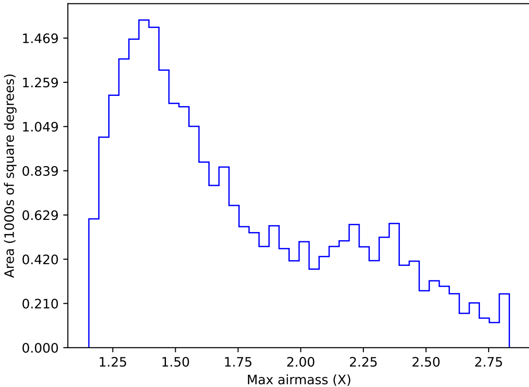
too_ignore_5_4v3.4_10yrs Yr 1 z band: Max airmass
