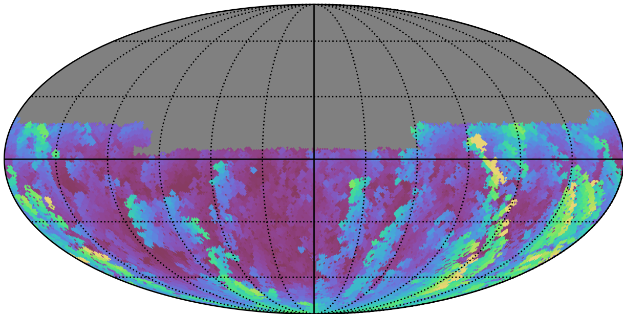
too_ignore_5_4v3.4_10yrs Yr 1 u band: Max airmass
