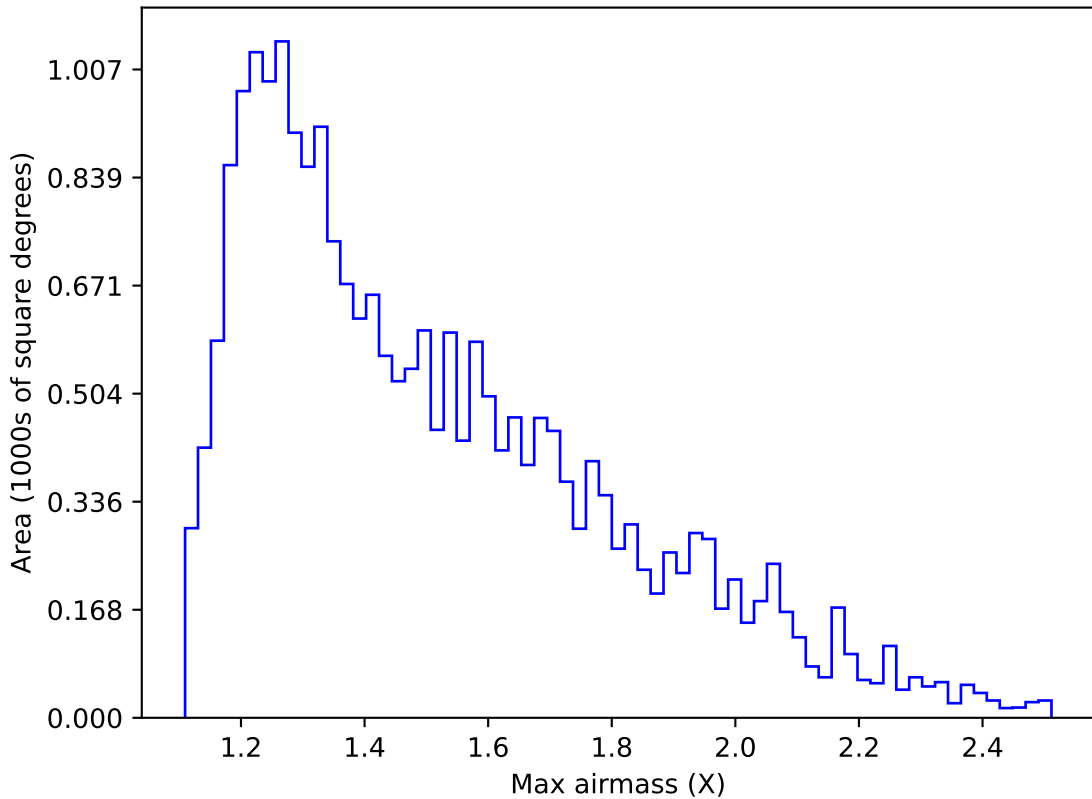
too_ignore_5_4v3.4_10yrs Yr 1 u band: Max airmass
