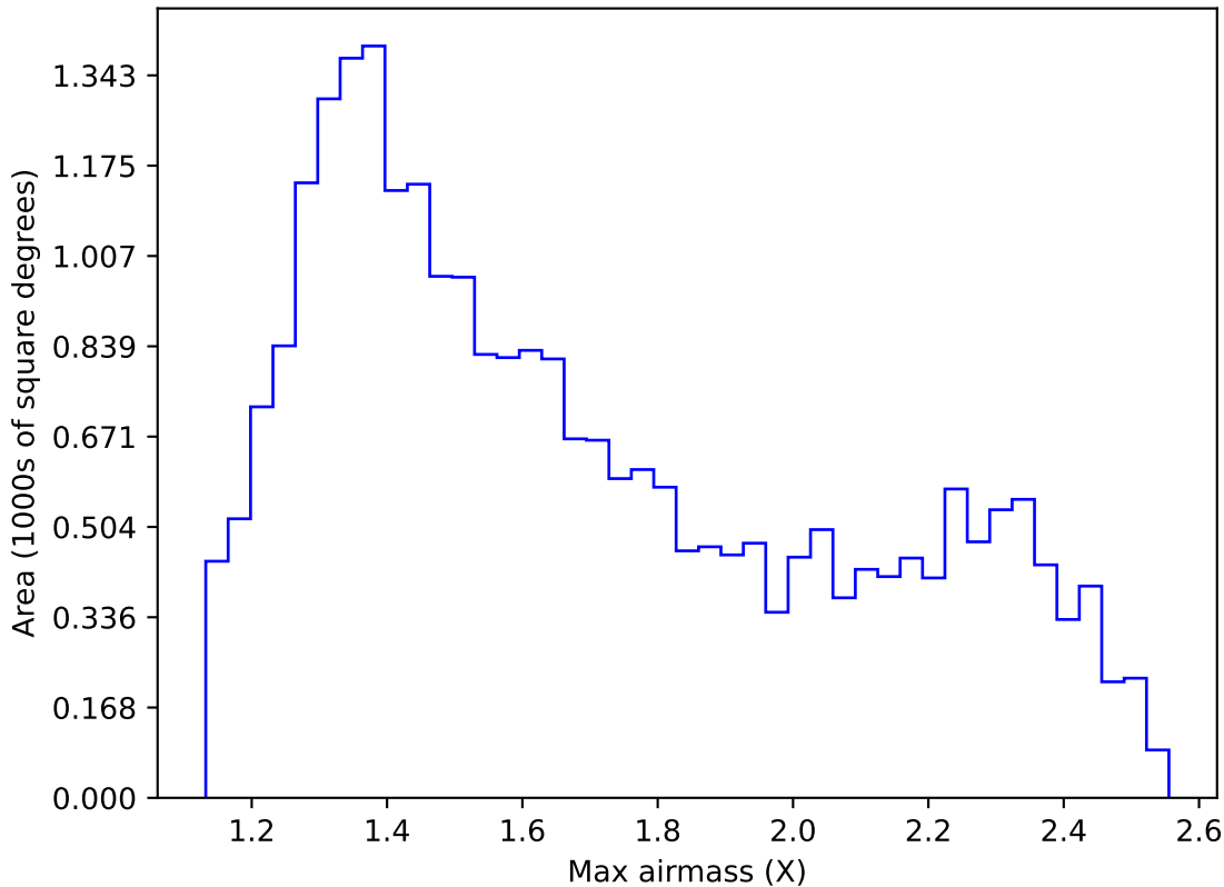
too_ignore_5_4v3.4_10yrs Yr 1 r band: Max airmass
