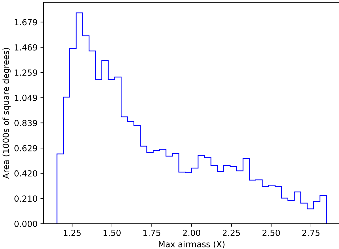
too_ignore_5_4v3.4_10yrs Yr 1 i band: Max airmass
