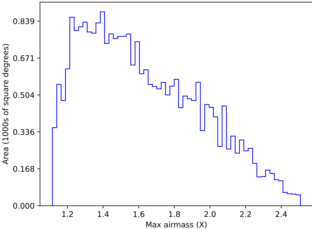
too_ignore_5_4v3.4_10yrs Yr 1 g band: Max airmass
