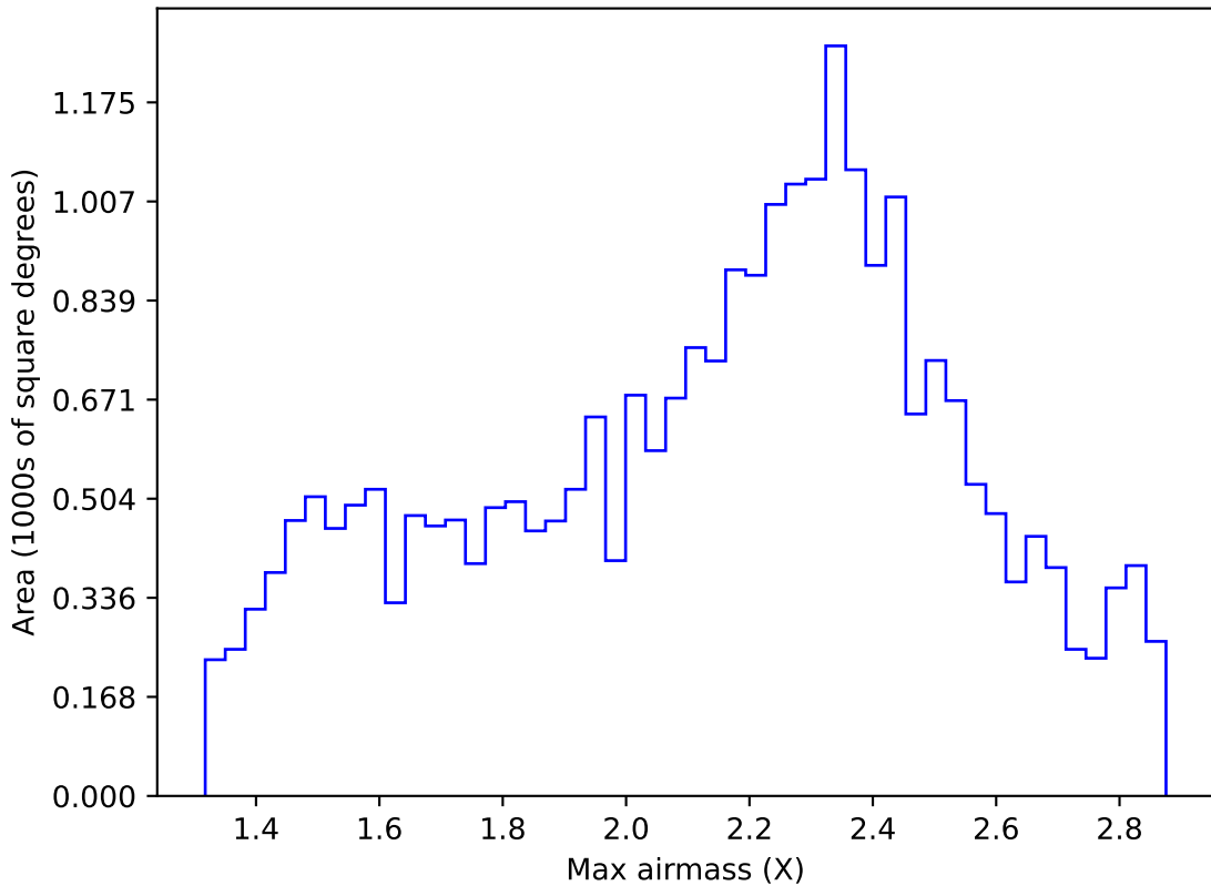
too_ignore_5_4v3.4_10yrs Yr 1 all bands: Max airmass
