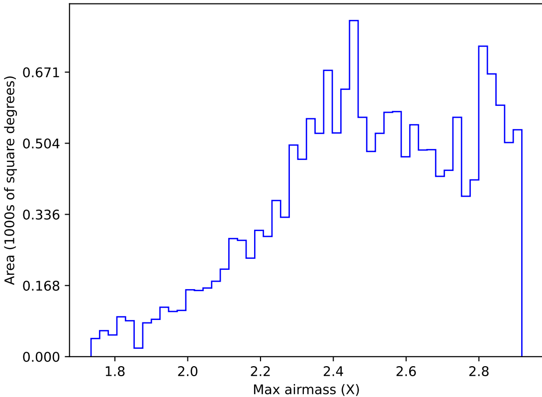
too_ignore_5_4v3.4_10yrs WFD z band: Max airmass
