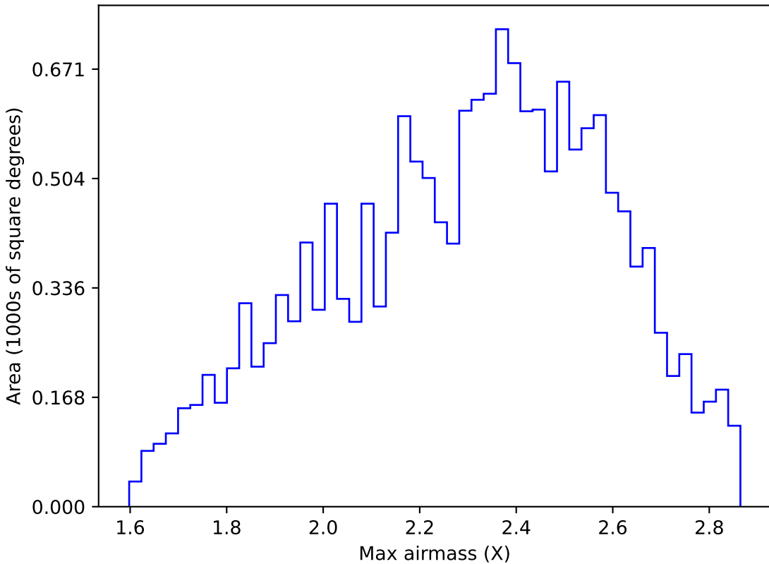
too_ignore_5_4v3.4_10yrs WFD y band: Max airmass
