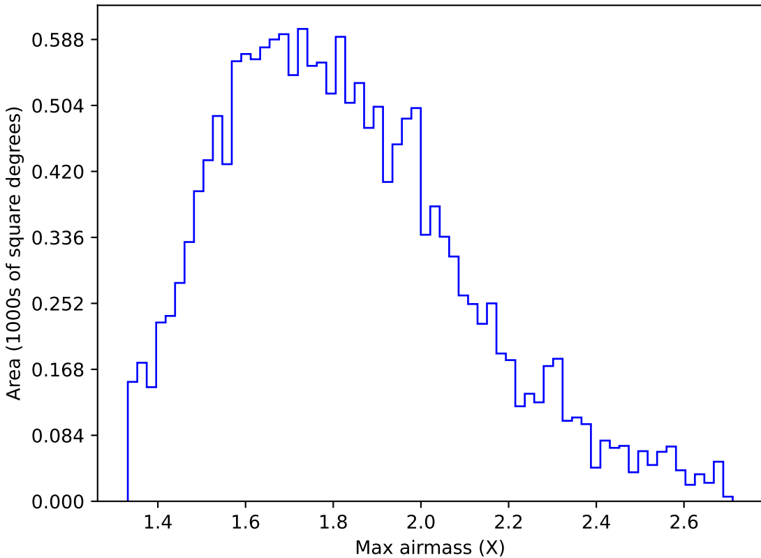
too_ignore_5_4v3.4_10yrs WFD u band: Max airmass
