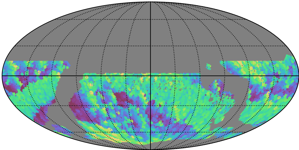
too_ignore_5_4v3.4_10yrs WFD r band: Max airmass
