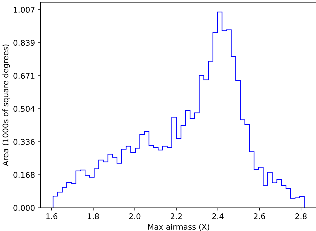
too_ignore_5_4v3.4_10yrs WFD r band: Max airmass
