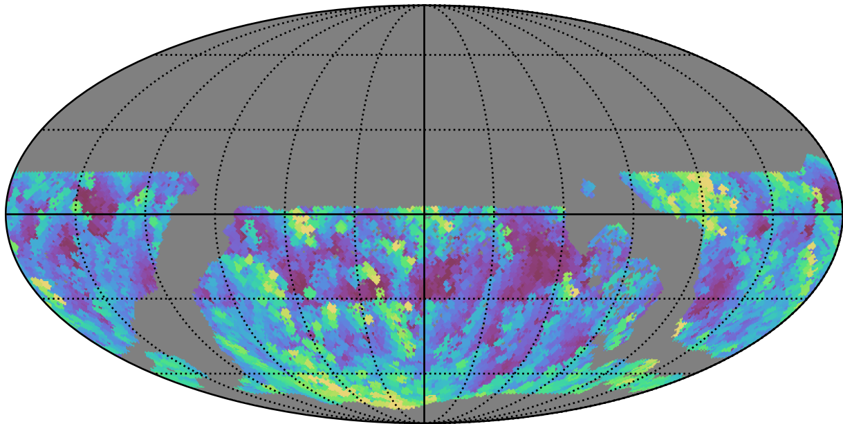
too_ignore_5_4v3.4_10yrs WFD g band: Max airmass
