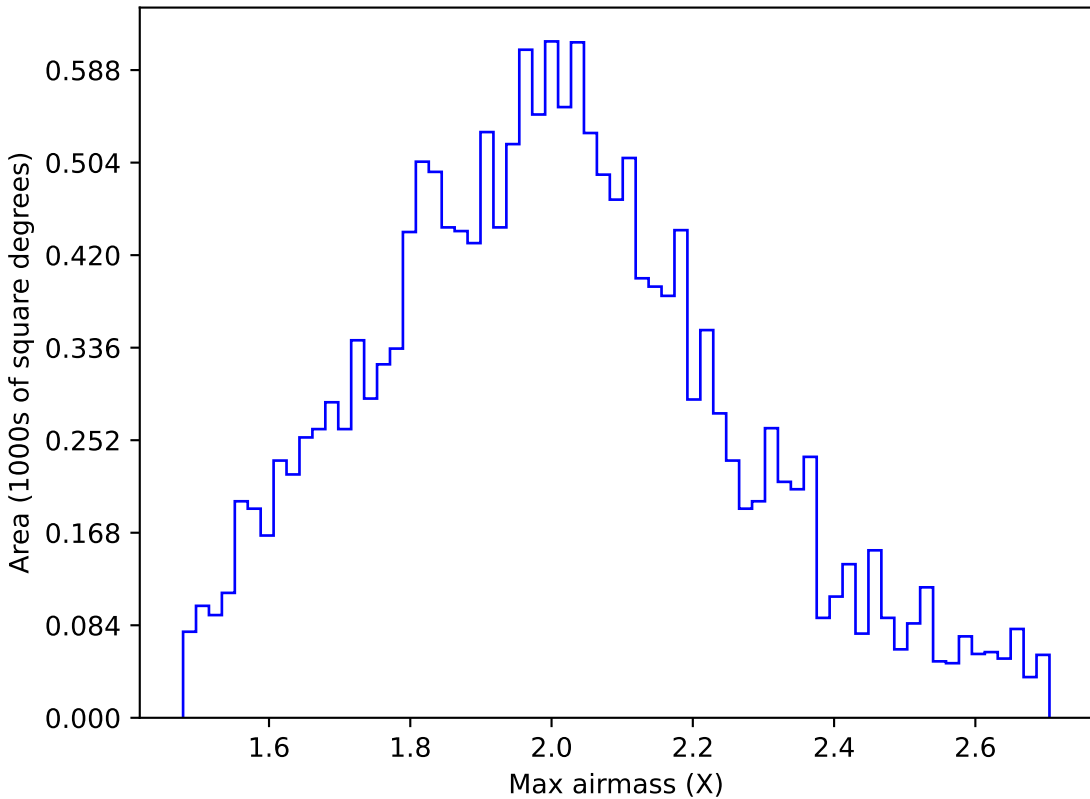
too_ignore_5_4v3.4_10yrs WFD g band: Max airmass
