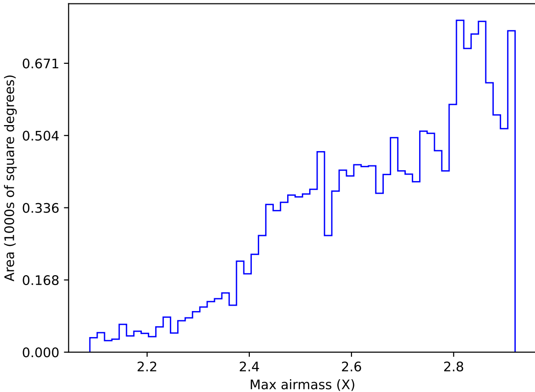
too_ignore_5_4v3.4_10yrs WFD all bands: Max airmass
