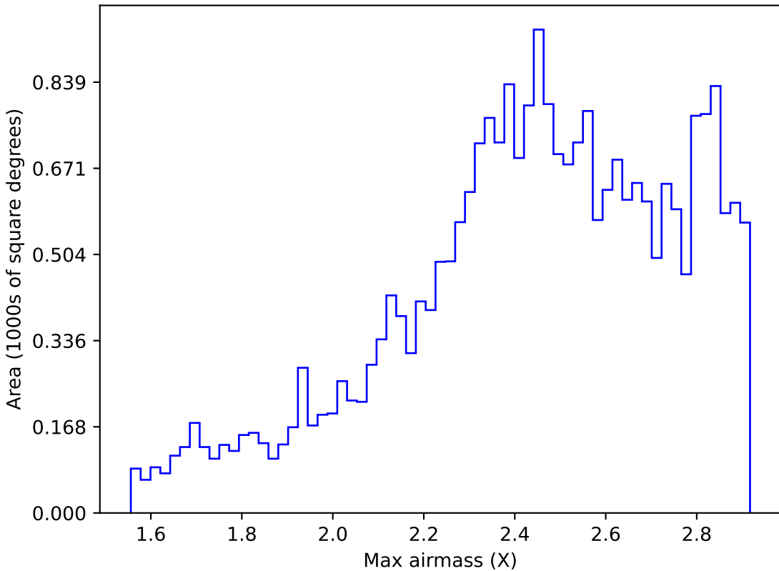
too_ignore_5_4v3.4_10yrs All sky z band: Max airmass
