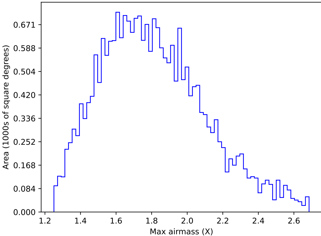
too_ignore_5_4v3.4_10yrs All sky u band: Max airmass
