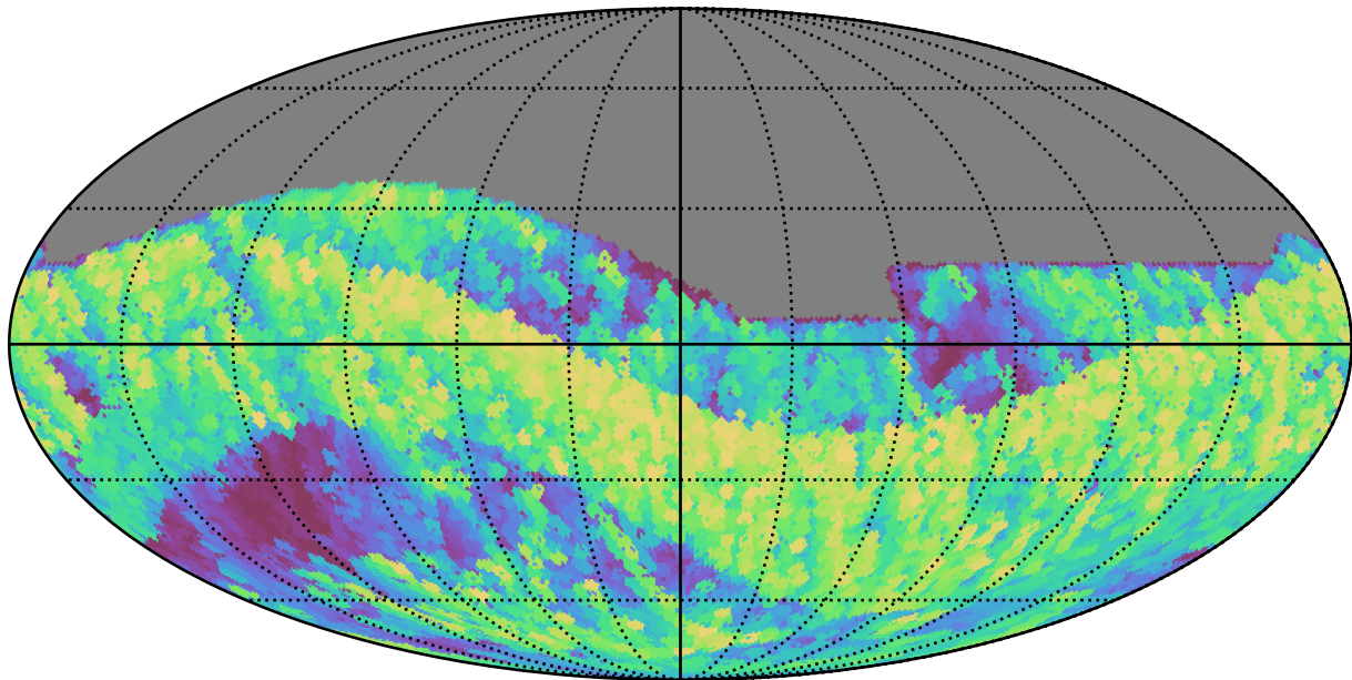
too_ignore_5_4v3.4_10yrs All sky i band: Max airmass
