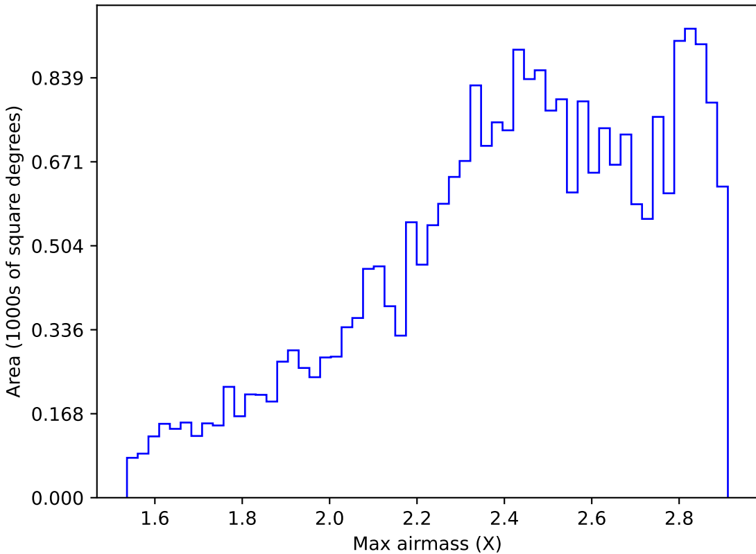
too_ignore_5_4v3.4_10yrs All sky i band: Max airmass
