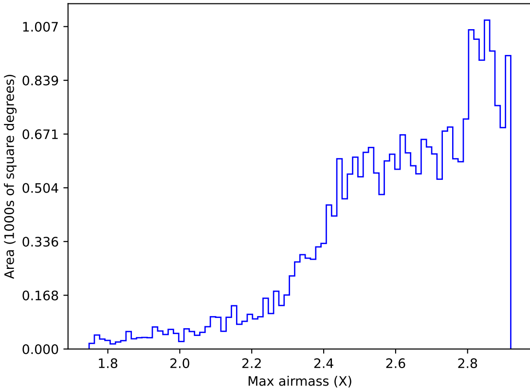
too_ignore_5_4v3.4_10yrs All sky all bands: Max airmass
