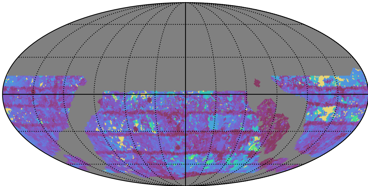
too_ignore_5_4v3.4_10yrs WFD z band: Max Inter-Night Gap
