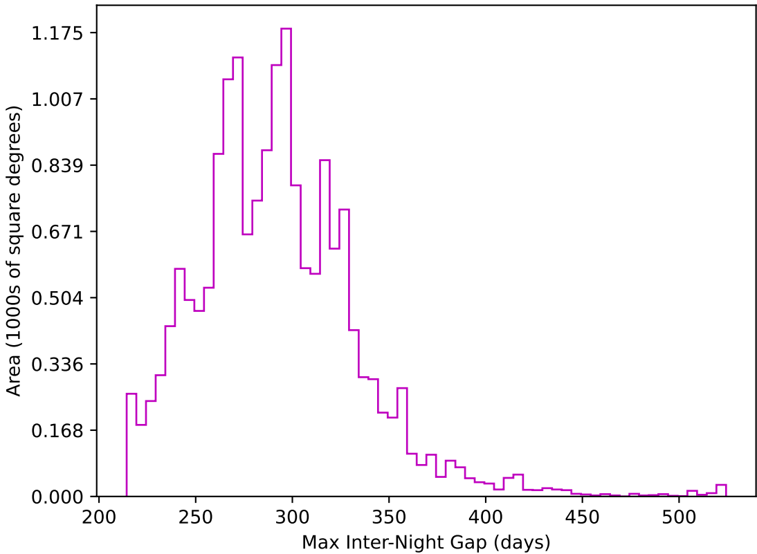
too_ignore_5_4v3.4_10yrs WFD z band: Max Inter-Night Gap
