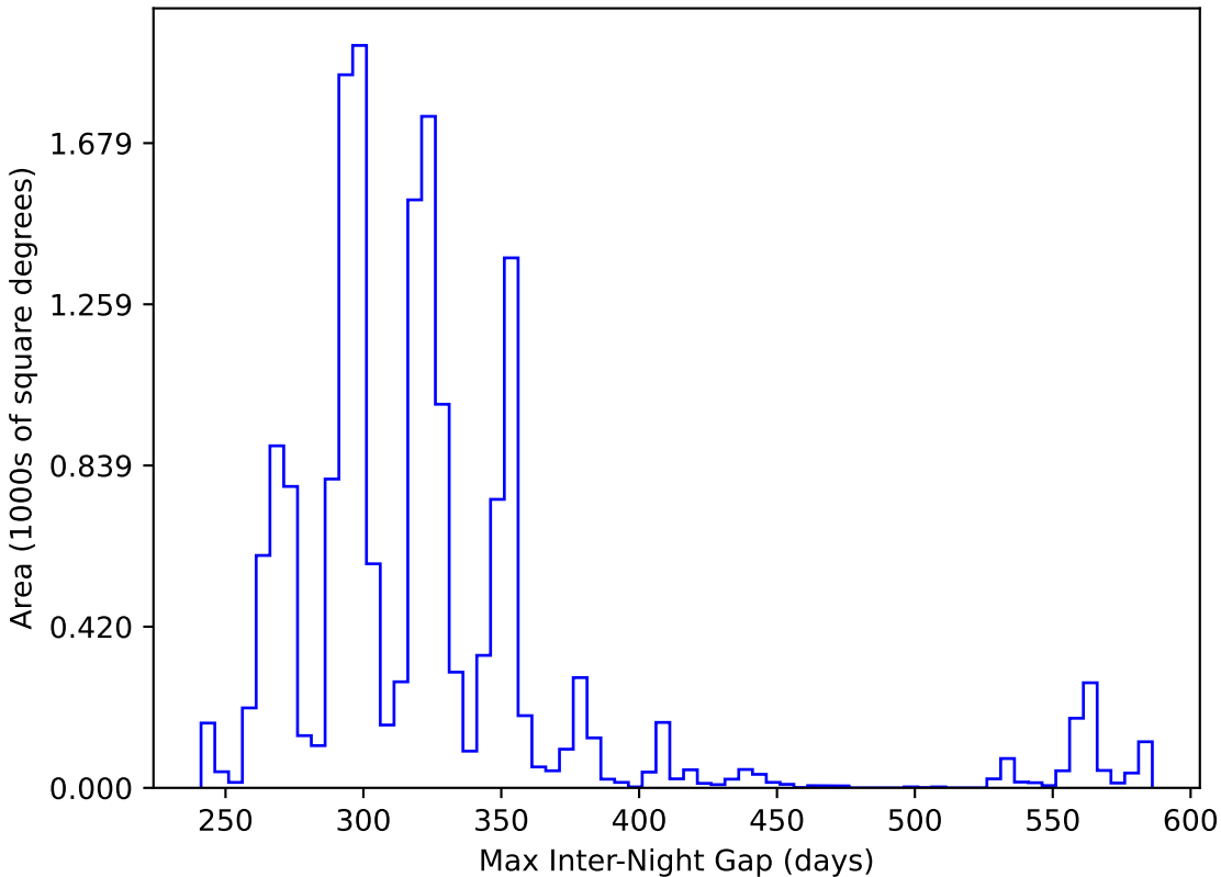
too_ignore_5_4v3.4_10yrs WFD y band: Max Inter-Night Gap
