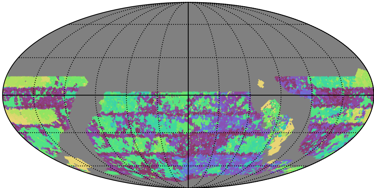
too_ignore_5_4v3.4_10yrs WFD u band: Max Inter-Night Gap
