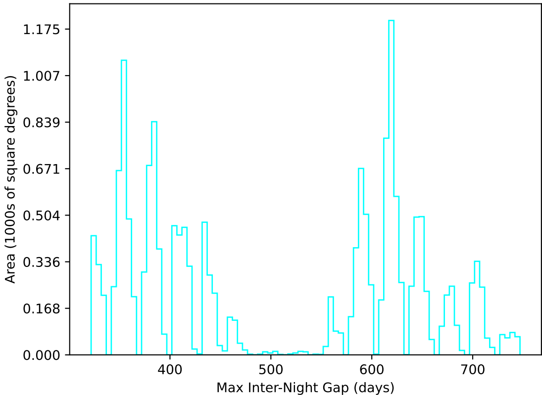
too_ignore_5_4v3.4_10yrs WFD u band: Max Inter-Night Gap
