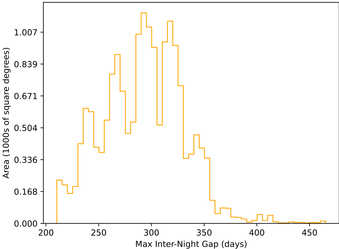
too_ignore_5_4v3.4_10yrs WFD r band: Max Inter-Night Gap
