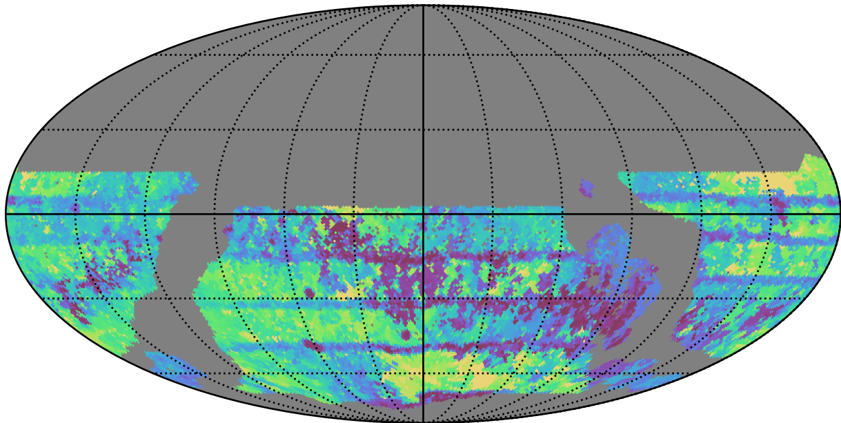
too_ignore_5_4v3.4_10yrs WFD all bands: Max Inter-Night Gap
