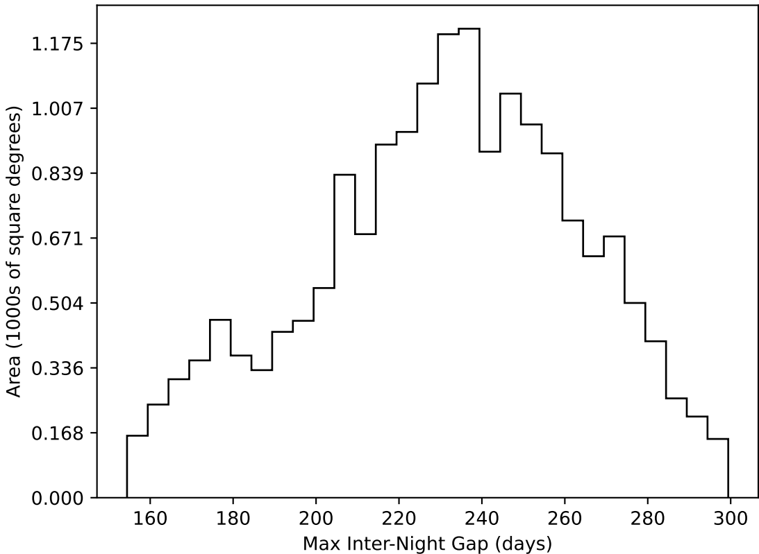
too_ignore_5_4v3.4_10yrs WFD all bands: Max Inter-Night Gap
