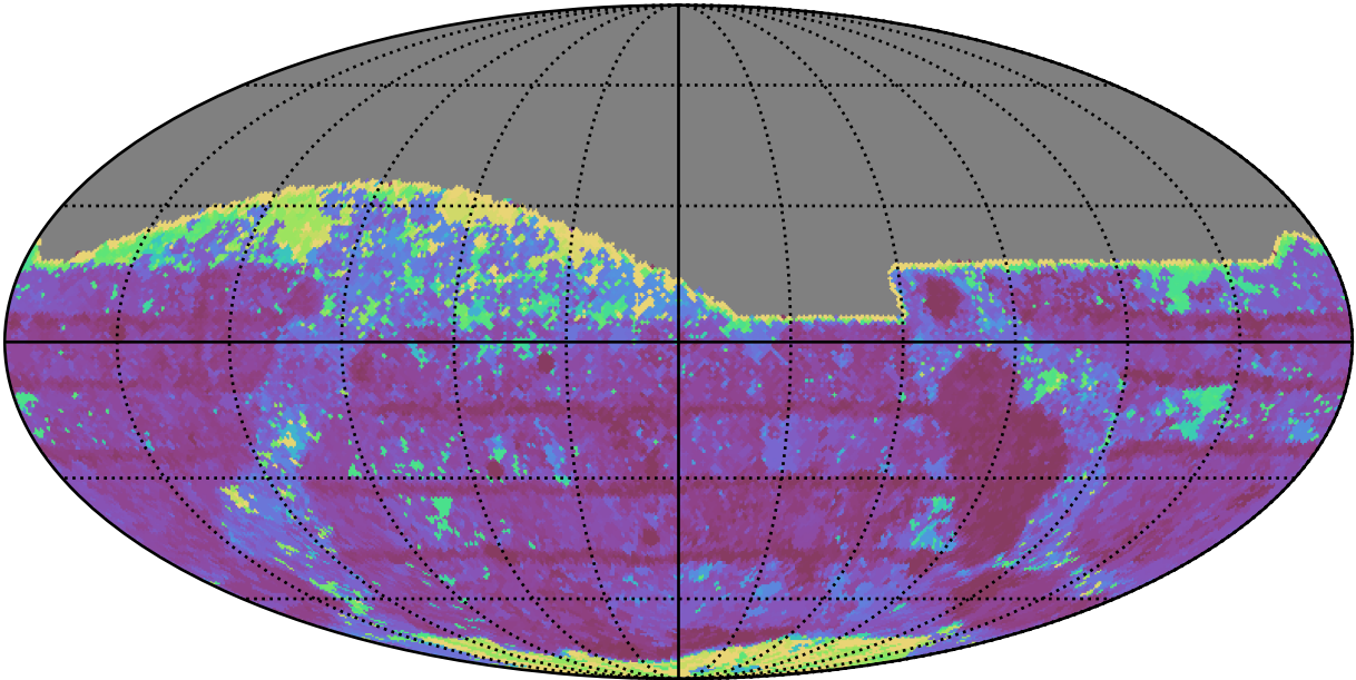
too_ignore_5_4v3.4_10yrs All sky z band: Max Inter-Night Gap
